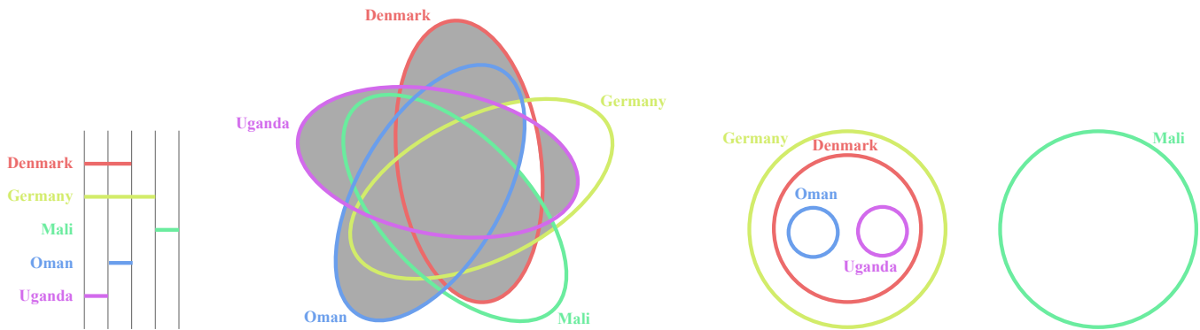
Figure 1: Diagrams obtained from translating textual statements: (left to right) linear, Venn, and Euler.
